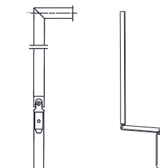
Kurbelstange fest
